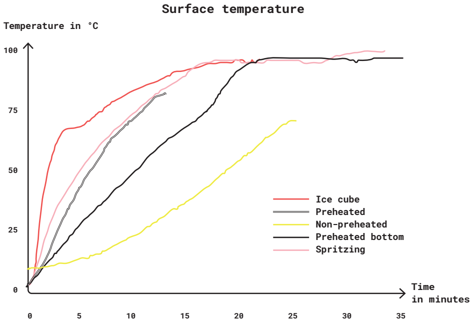
Figure 11.16: A chart showing how the temperature of the surface of the apple changes with different steaming techniques.
