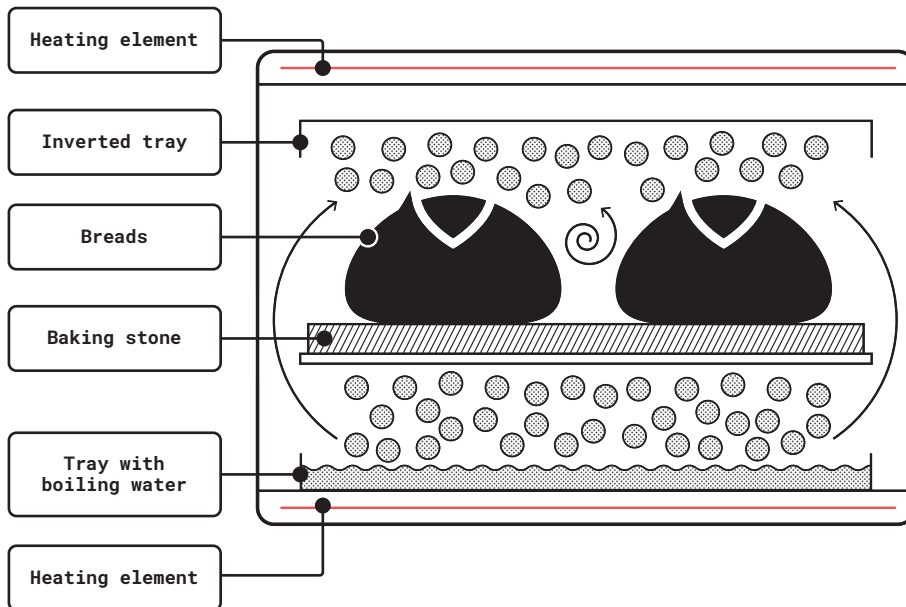
Figure 9.3: How steam builds in your oven using the late-described inverted tray method.
