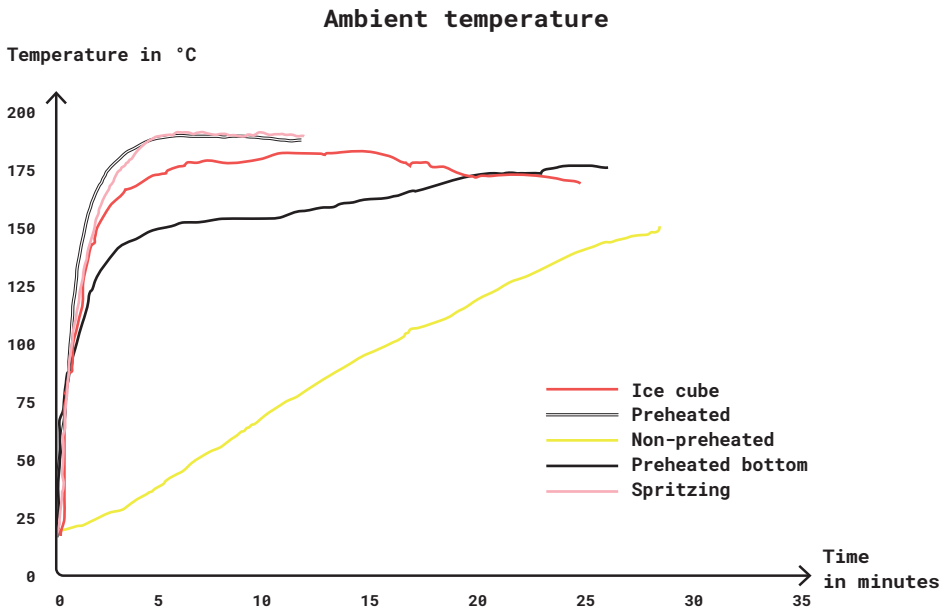
Figure 11.17: This figure shows how the ambient temperatures inside of the Dutch oven change depending on the steaming technique that is used.
